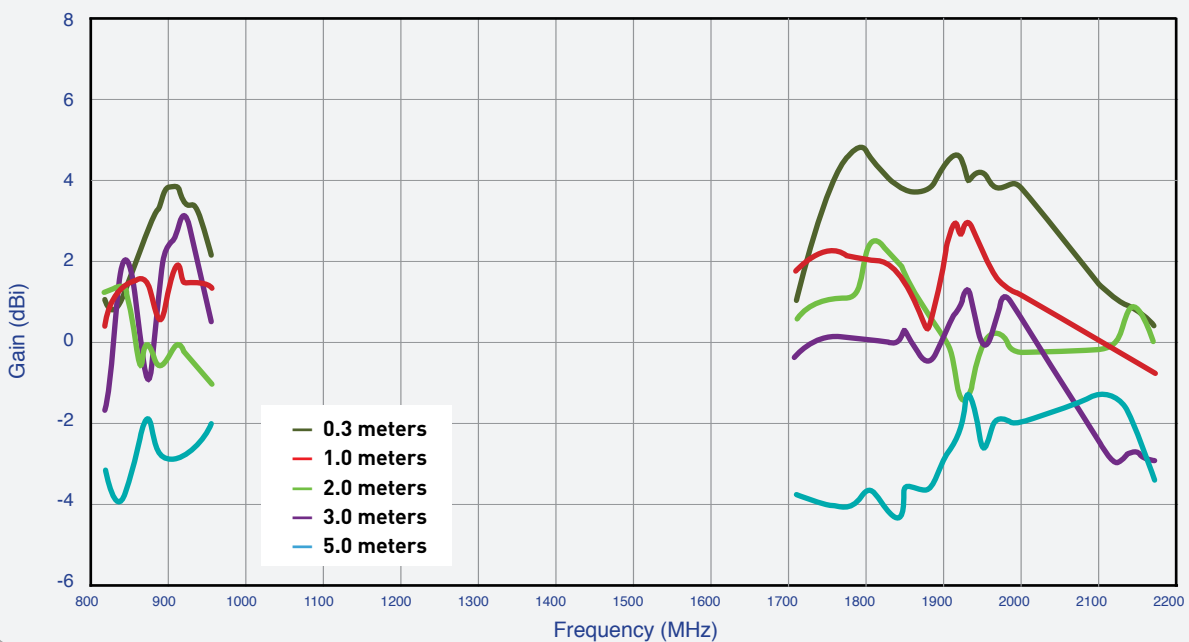
Figure 9. Gain of the MA105 antenna on 30*30cm metal plate
