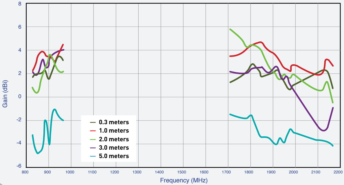
Figure 8. Gain of the MA105 antenna in free space
