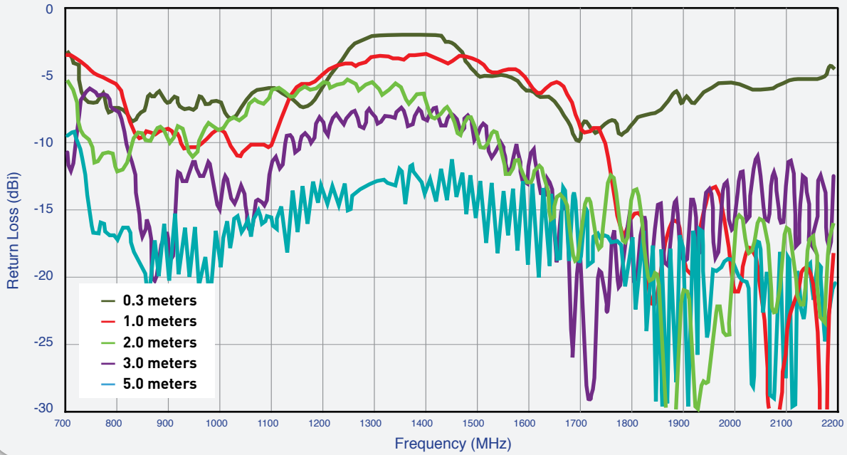
Figure 2. Return Loss of the MA105 antenna in free space
