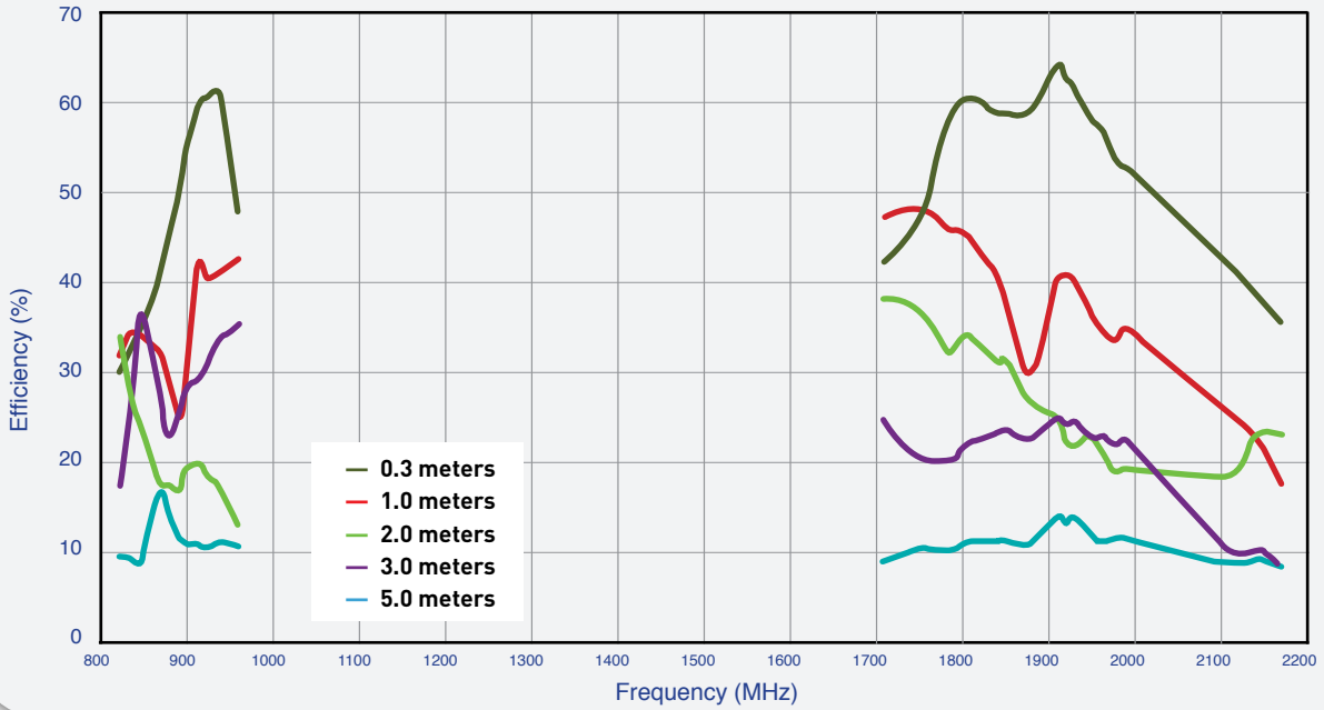
Figure 6. Efficiency of the MA105 antenna on 30*30cm metal plate.
