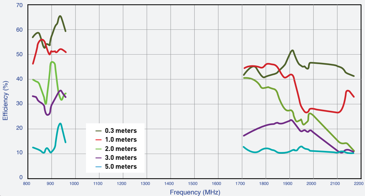
Figure 5. Efficiency of the MA105 antenna in free space.
