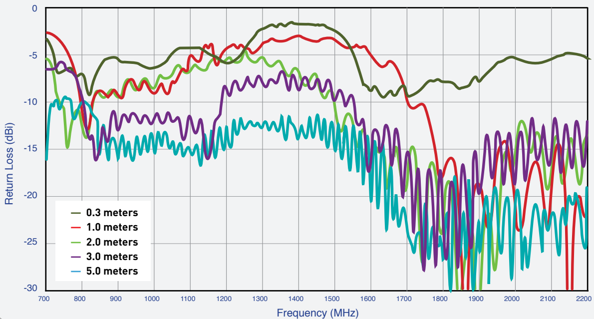
Figure 3. Return Loss of the MA105 antenna on 30*30cm metal plate
