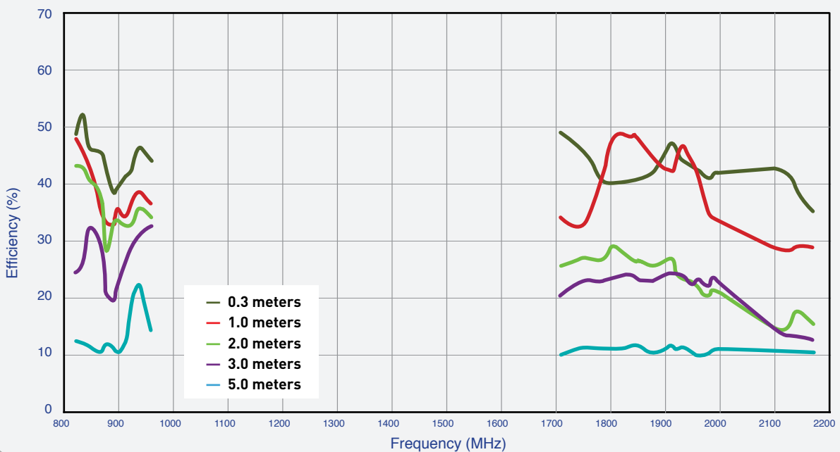
Figure 7. Efficiency of the MA105 antenna on 60*60cm metal plate.
