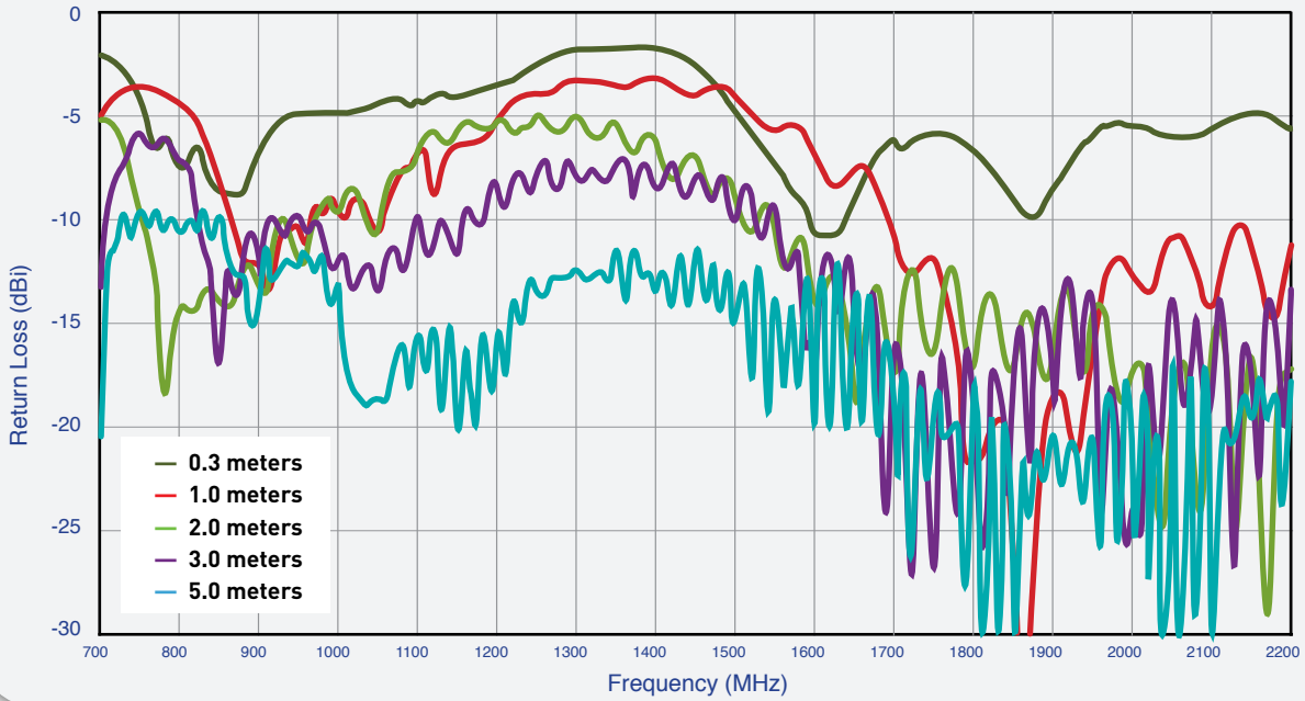
Figure 4. Return Loss of the MA105 antenna on 60*60cm metal plate.
